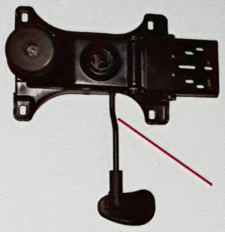
SYNCHRO (LIGHT, 65MM, 75MM)
